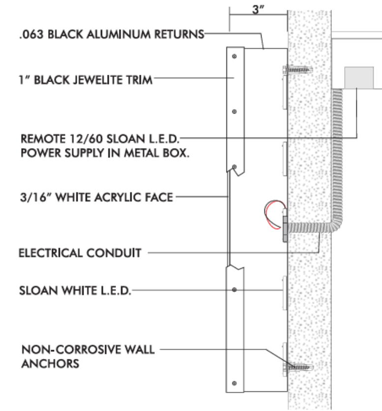
B SECTION DETAIL FACE LIGHTED CHANNEL LETTERS
