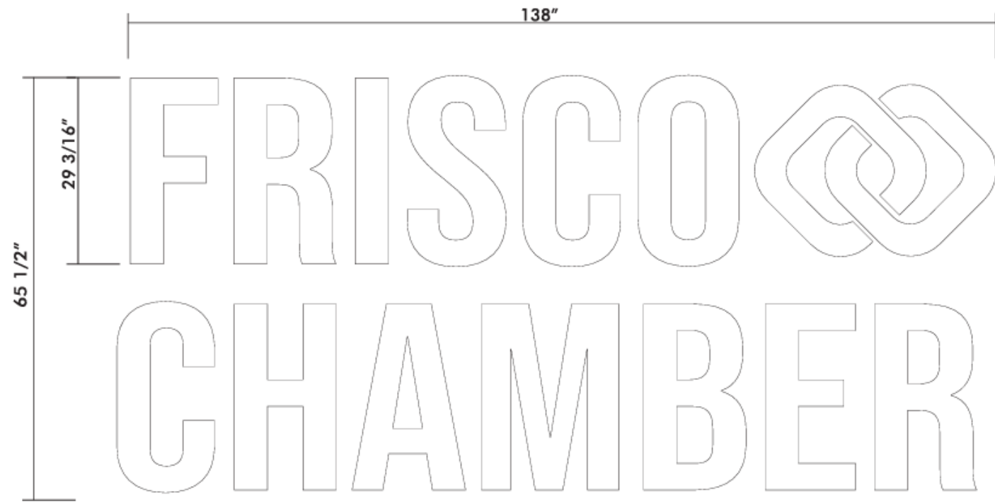
A FACE LIGHTED CHANNEL LETTERS QTY: 1
